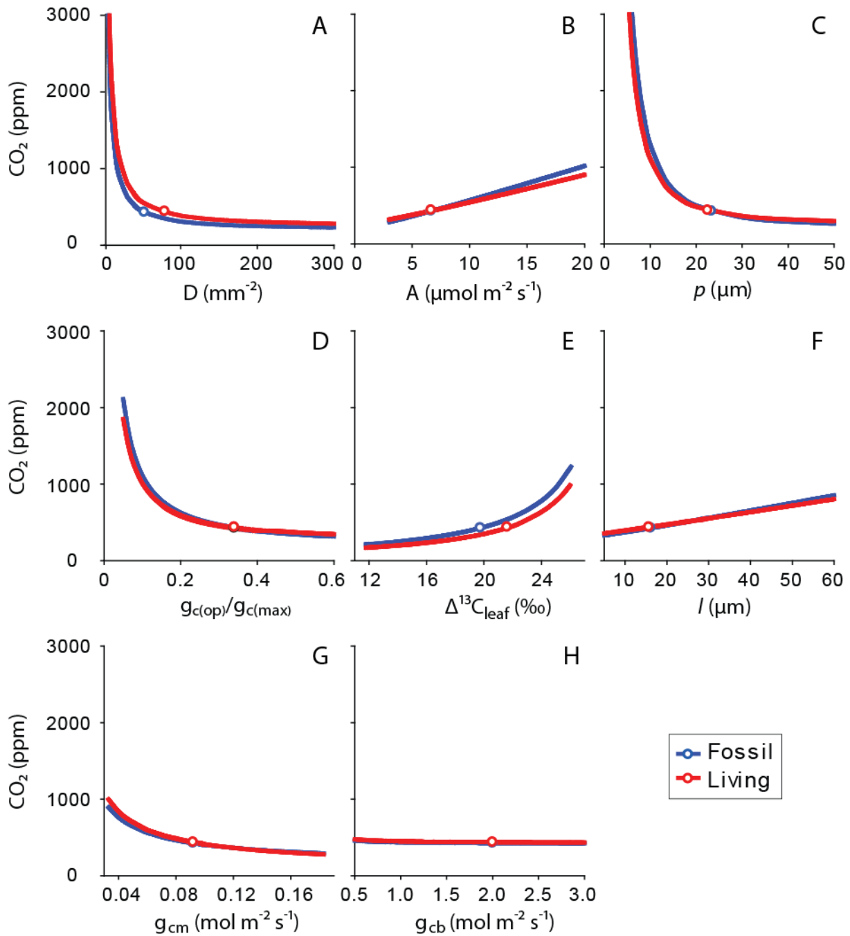
Figure DR3. Sensitivity of input parameters on calculated \text{CO}_2 following the Franks et al. (2014) model. The range in all input parameters are representative of \text{C}_3 plants. The blue circles are the site-mean values for Napartulik; the red circles are the mean values for extant Metasequoia . Along each curve, only one input parameter was varied; all others are held fixed at their measured or modeled means. A. D = stomatal density B. A = photosynthetic rate C. p = pore length D. g_{c(\text{op})}/g_{c(\text{max})} = scaling between operational and maximum stomatal conductance E. \Delta^{13}\text{C}_{\text{leaf}} = photosynthetic fractionation F. l = stomatal pore depth G. g_{\text{cm}} = mesophyll conductance H. g_{\text{cb}} = boundary layer conductance.
