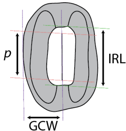
Figure DR8. Illustration of stomatal measurements taken on fossil and living Metasequoia . The shaded grey portion represents what is covered by the overarched epidermal cells and not visible in map view using epifluorescence (see Fig. DR7). p = pore length. IRL = inner rectangular length. GCW = single guard cell width. For fossils, IRL was most readily accessible to measure and was used to scale to p and GCW .
