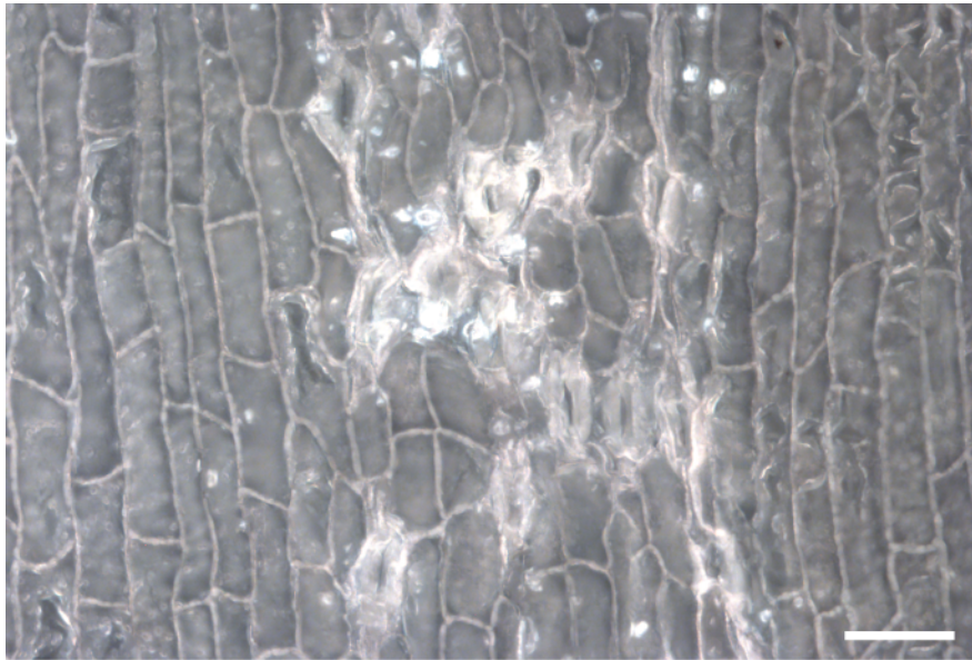
Figure DR6. Cuticle of M. occidentalis cleared of mesophyll from Napartulik fossil forest layer C. Image shows internal surface of cuticle under epifluorescence light. Scale bar = 50 \mu\text{m} .
